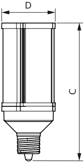
Corn lamp LED 54W EX39 850 CL
