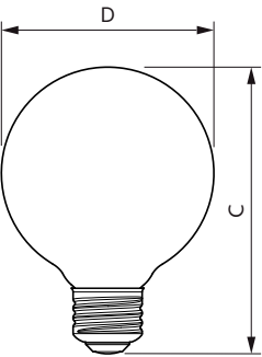
Candle G25 120V3.8-40W350lm5000KE26DCL
