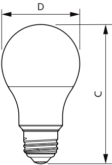
Bulb A60 120V 6-40W 450lm 5000K E26 ND
