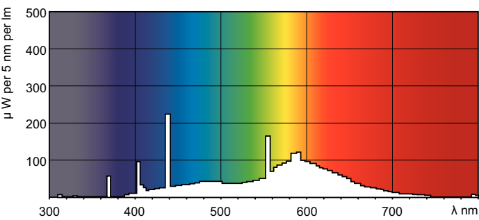
LDPO_TL-MINI_33-640-Spectral power distribution Colour
