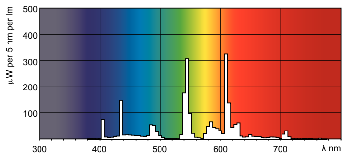
LDPO_PLLXEW_835-Spectral power distribution Colour
