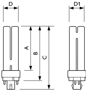
PL-C XEW 18W/841/4P ALTO 14W
