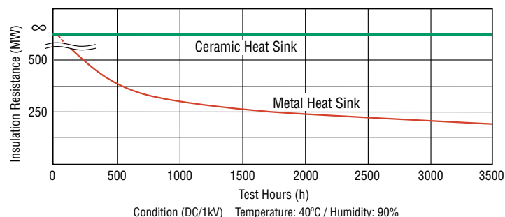
Insulation Resistance for Ceramic & Metal Bases
