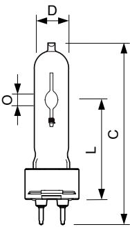
CDM-T Elite 70W/930 G12
