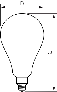
Bulb A160 120V 8-40W 450lm 2000K E26 D
