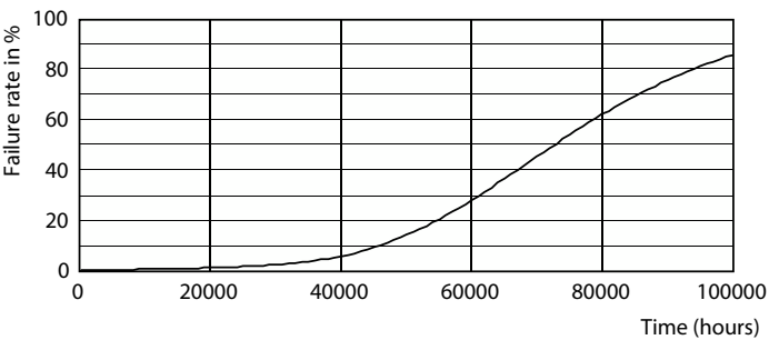
Life Expectancy Diagram - 10T8/COR/48-850/DF16/G/DIM UL-C 25/1
