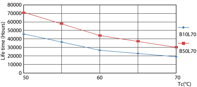
Lumen Maintenance Diagram - 10T8/COR/48-850/DF16/G/DIM UL-C 25/1
