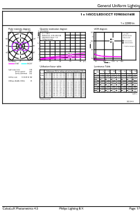
General uniform lighting - 145CC/LED/3CCT/LS EX39 BB 3/1
