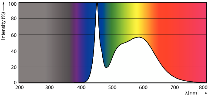
Spectral Power Distribution Colour - 145CC/LED/3CCT/LS EX39 BB 3/1
