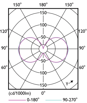
Light Distribution Diagram - 145CC/LED/3CCT/LS EX39 BB 3/1
