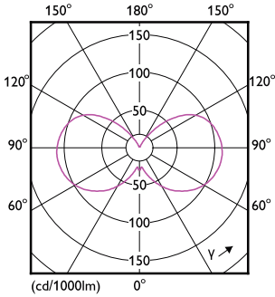
Light Distribution Diagram - 5BA11/PER/UD50/CL/G/E26/D 6/3PF T20
