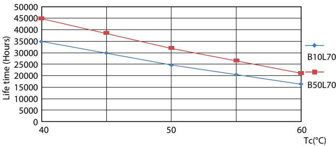
Life Expectancy Diagram - 8PL-C/T/COR/26V-3CCT/MF10/P/20/1
