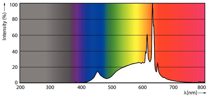
LEDbulb T20 8,8W A19 E26 927 FR-POC
