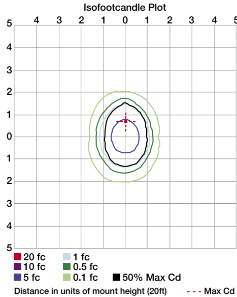
ISO Footcandle plot 75W ISO FC_15ft
