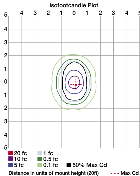
ISO Footcandle plot 90W ISO FC_15ft
