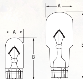
Wedge Base
