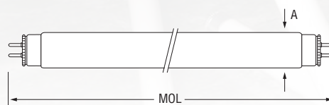
Bi-Pin G5 Base
