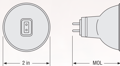
GU5.3 Base
