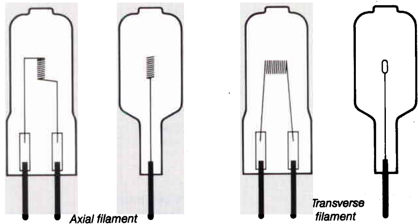
7 Tungsten halogen LV lamps with axial and transverse filaments
